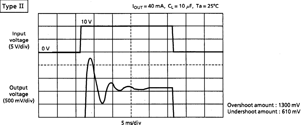
Figure 17 Type II ringing waveform
