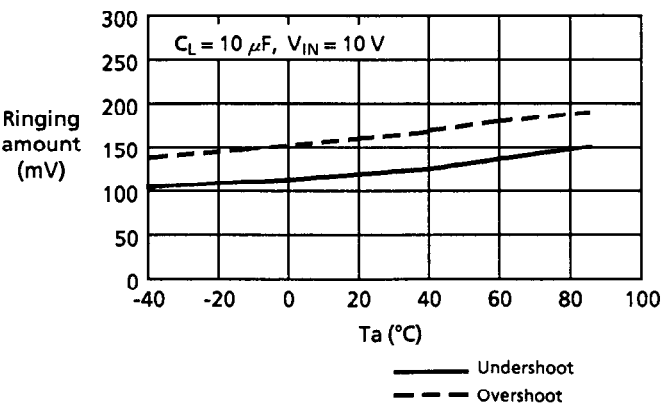
4. Temperature dependency
