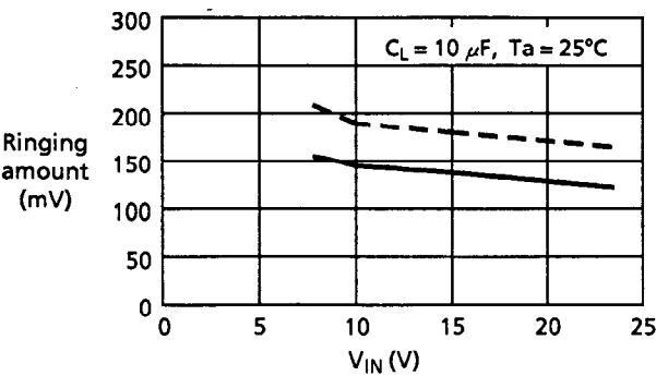
3. V_{IN} dependency
