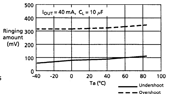
4. Temperature dependency
