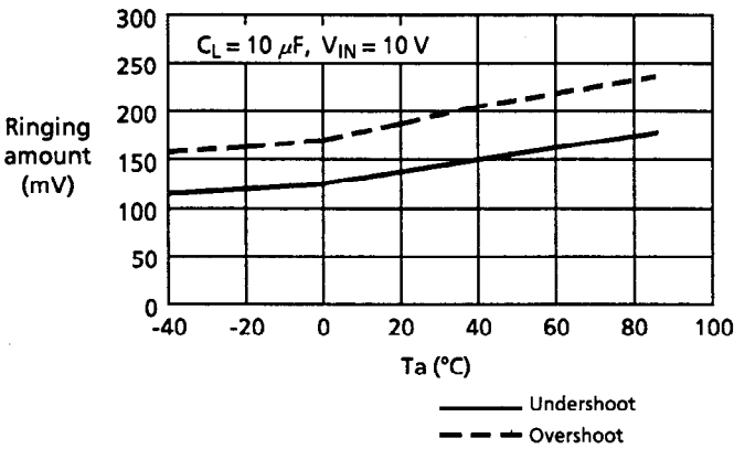
4. Temperature dependency
