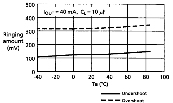
4. Temperature dependency
