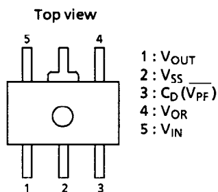
Figure 1 Pin assignment
