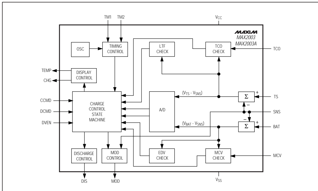
Figure 2. Block Diagram
