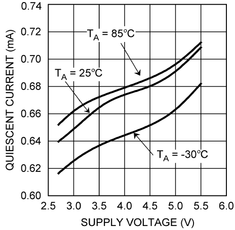
Quiescent Current vs Supply Voltage ( V_{CON} = 0.267V , FB = 2V , No Load)
