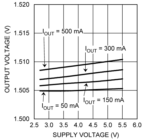
Output Voltage vs Supply Voltage ( V_{OUT} = 1.5V , V_{CON} = 0.5V )
