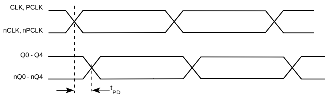
FIGURE 6 - PROPAGATION DELAY
