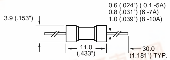
672 000 Series
