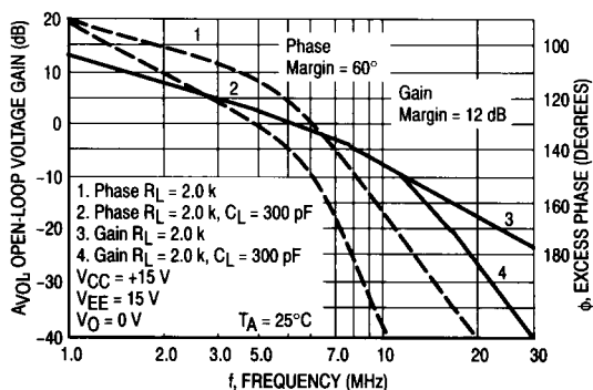
Figure 19. Open-Loop Voltage Gain and Phase versus Frequency
