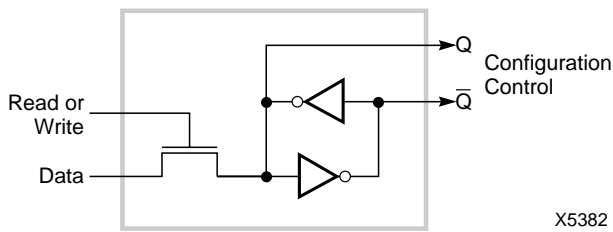
Figure 3: Static Configuration Memory Cell.
