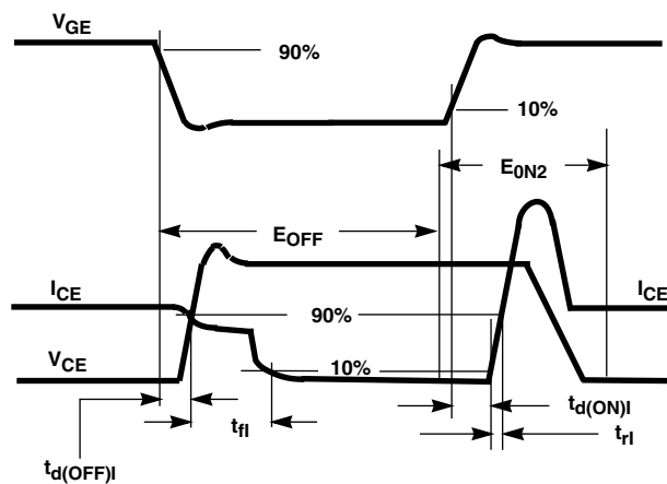
FIGURE 25. SWITCHING TEST WAVEFORMS
