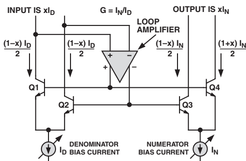
Figure 2. The Basic Core of the AD8330
