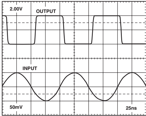
TPC 37. Overdrive Response, V_{DBS} = 1.5\text{ V} , V_{MAG} = 0.5\text{ V} , 18.5 dB Overdrive
