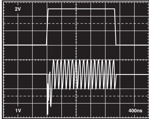
TPC 38. ENBL Interface Response. Top: V_{ENBL} ; Bottom: V_{OUT} , f = 10\text{ MHz}
