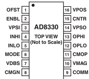
16-Lead QSOP
