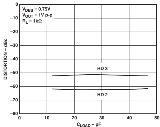
TPC 21. Harmonic Distortion vs. C_{LOAD}
