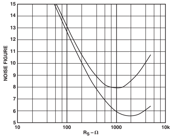
Figure 10. Noise Figure for Source Resistance of 50 Ω to 5 kΩ, at f = 10 MHz (lower) and 100 MHz (Simulation)
