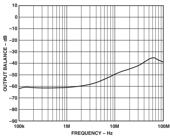
TPC 11. Output Balance Error vs. Frequency for a Representative Part
