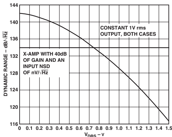
Figure 11. Dynamic Range in \text{dB}/\sqrt{\text{Hz}} vs. V_{DBS} ( V_{MAG} = 0.5\text{ V} , 1\text{ V rms output} ) Compared with a Representative X-AMP (Simulation)
