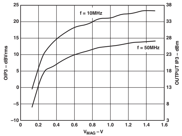
TPC 29. Output IP3 vs. V_{MAG}
