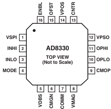
16-Lead LFCSP
