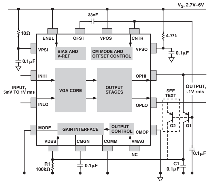
Figure 21. Simple AGC Amplifier (Preliminary)
