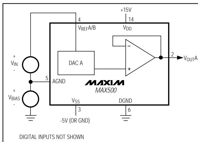
Figure 10. AGND Bias Circuit
