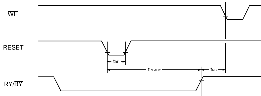
Figure 12 RESET, RY/ \overline{BY} Timing Diagram
