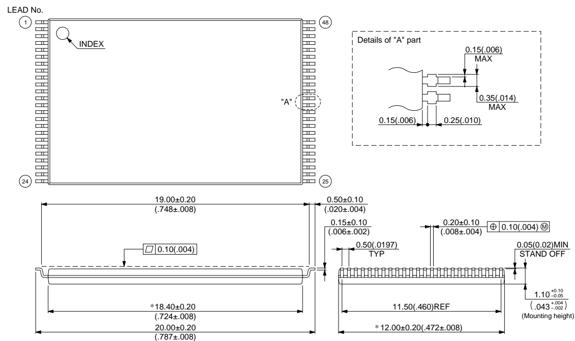
48-pin plastic TSOP(I) (FPT-48P-M20)
