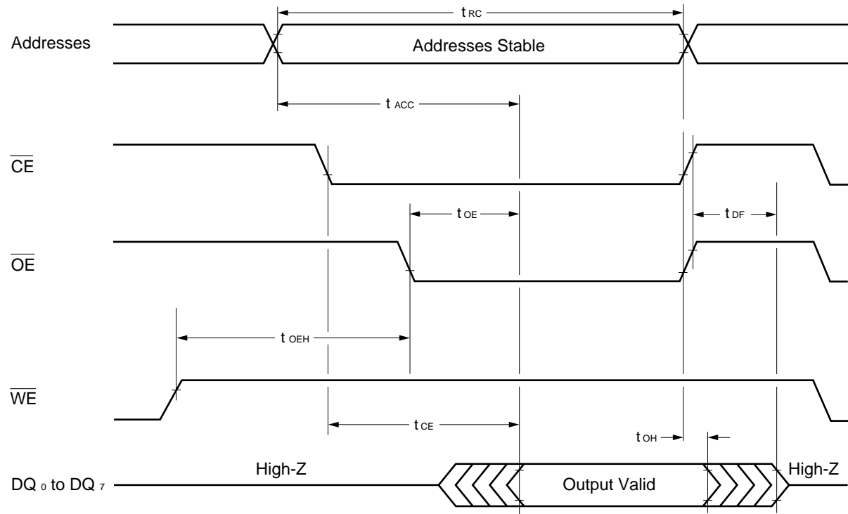
Figure 5.1 AC Waveforms for Read Operations
