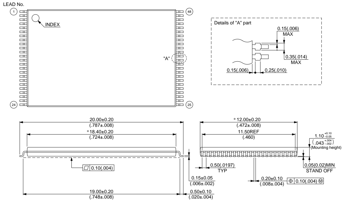
48-pin plastic TSOP(I) (FPT-48P-M19)
