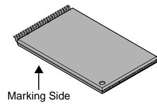
48-pin plastic TSOP(I)
