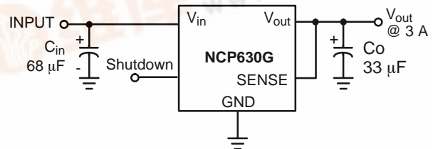
Figure 2. Typical Application Circuit for NCP630G
