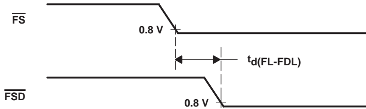
Figure 5–2. Slave \overline{\text{FS}} to \overline{\text{FSD}} Timing
