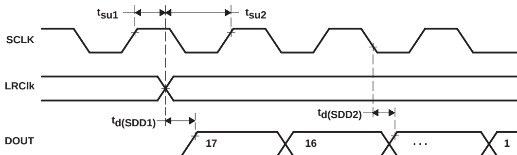
Figure 4-5. SCLK to LRClk and DOUT – Slave Mode 0, Fsync High
