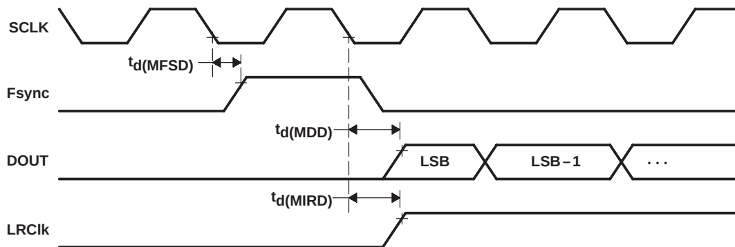
Figure 4-4. SCLK to Fsync, DOUT, and LRClk – Master Mode 7
