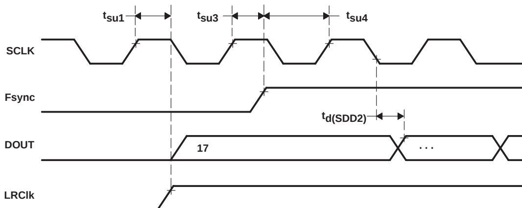
Figure 4-6. SCLK to Fsync, LRClk, and DOUT – Slave Mode 2, Fsync Controlled
