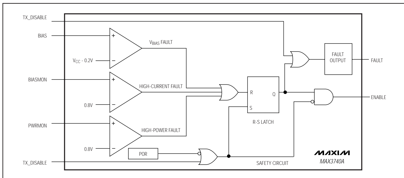
Figure 2. Safety Circuit
