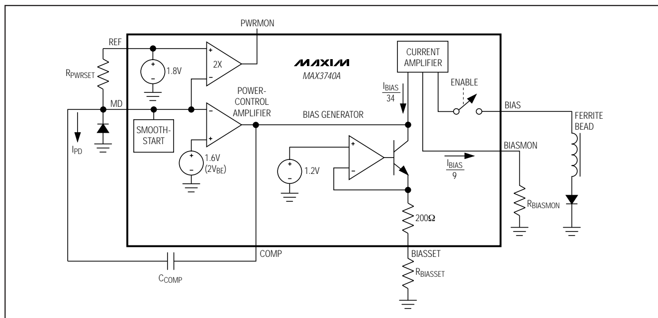
Figure 1. Bias Generator
