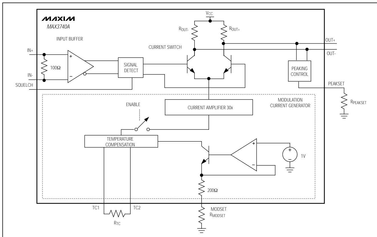
Figure 3. Modulation Circuit
