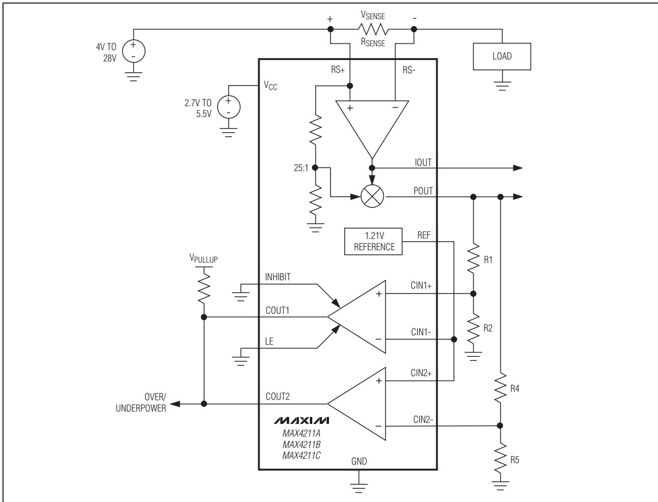
Figure 1. Window Comparator for Detecting Underpower and Overpower Faults (Also Detects Undercurrent and Overcurrent Faults by R1 and R4 to IOOUT Instead of POUT)
