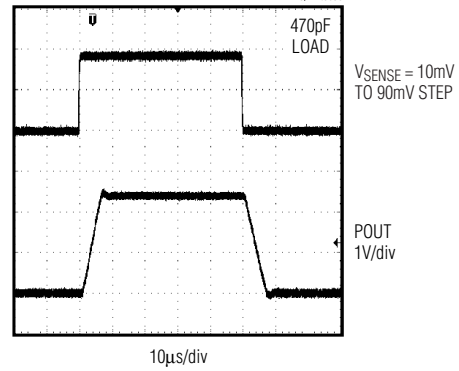
POUT LARGE-SIGNAL PULSE RESPONSE MAX4210/11 ttc35
