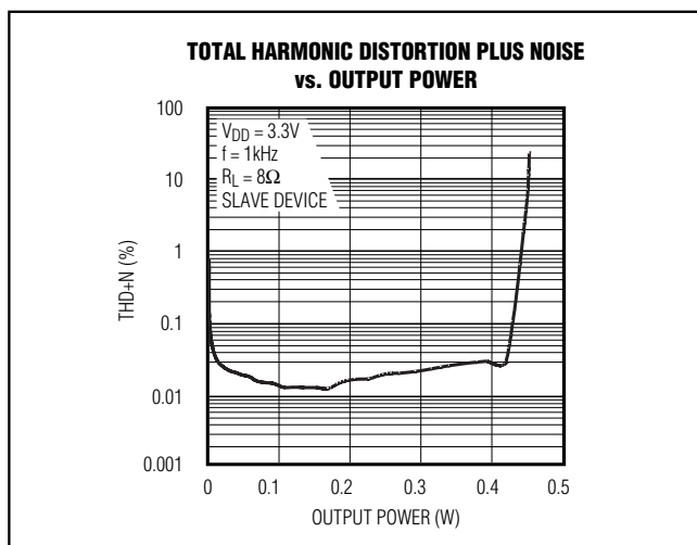
Figure 8. Master-Slave THD+N
