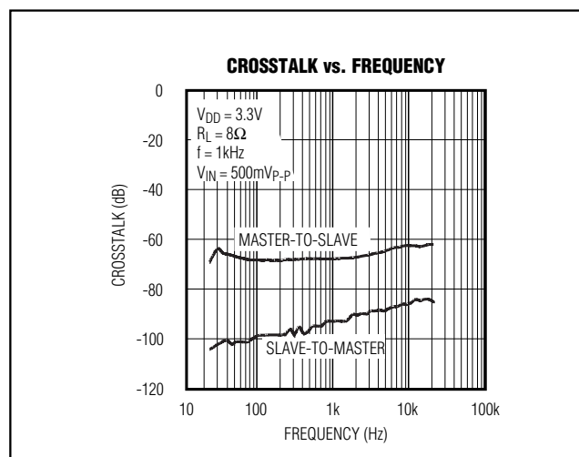
Figure 9. Master-Slave Crosstalk
