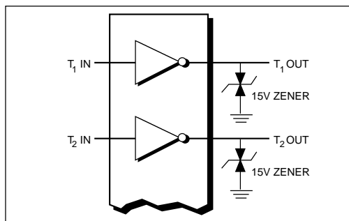
Figure 3. High Voltage Short Circuit Protection
