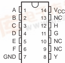
SN54ALS30A, SN54AS30 . . . J PACKAGE SN74ALS30A, SN74AS30 . . . D OR N PACKAGE (TOP VIEW)
