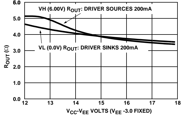
FIGURE 9. R_{OUT} vs DEVICE VOLTAGE
