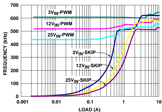
FIGURE 2. SWITCHING FREQUENCY vs LOAD ( T_{ON} = \text{GND} )
