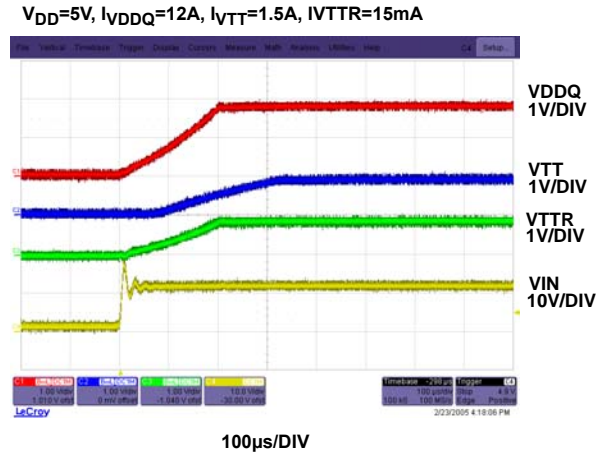
FIGURE 12. POWER-UP WAVEFORMS
