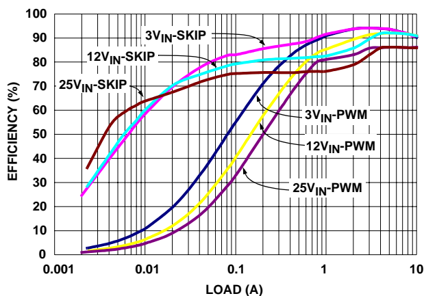
FIGURE 1. EFFICIENCY vs LOAD - 1.8V ( T_{ON} = \text{GND} )
