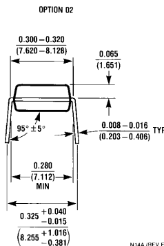
Molded Dual-In-Line Pkg. (N) Order Number LMC660AIN, LMC660CN or LMC660EN NS Package Number N14A
