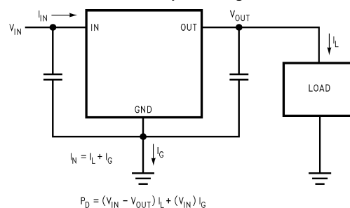
Power Dissipation Diagram
