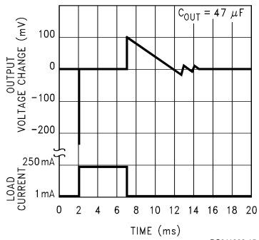
Load Transient
