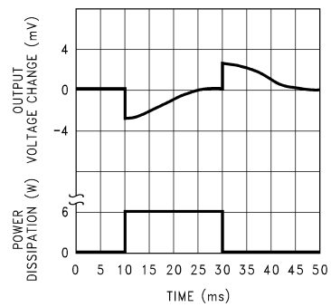
Thermal Regulation
