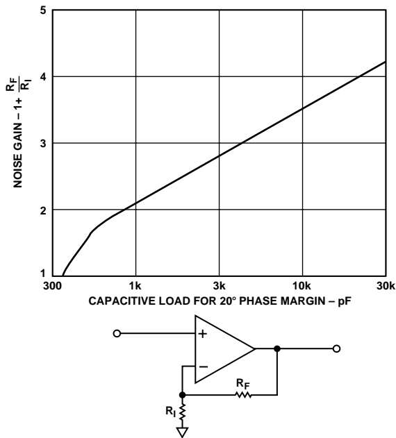
Figure 41. Capacitive Load Tolerance vs. Noise Gain
