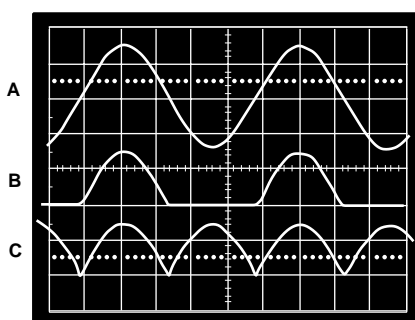
Figure 44. Single Supply Half- and Full-Wave Rectifier
