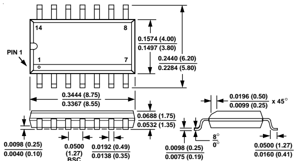
14-Pin Narrow Body SOIC Package (SO-14)
