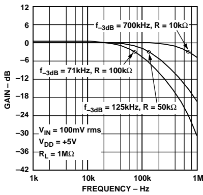
Figure 23. -3 dB Bandwidths
