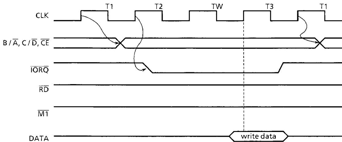
Figure 3.7 Write Timing
