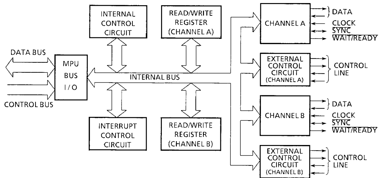
Figure 3.1 Block Diagram
