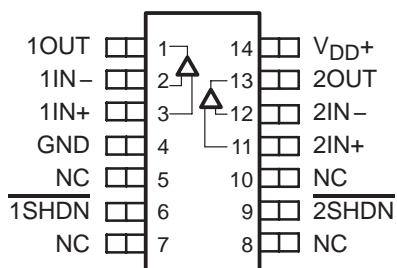
TLV2463 D OR PW PACKAGE (TOP VIEW)
