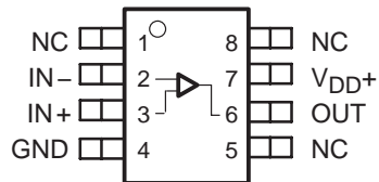
TLV2461 D OR PW PACKAGE (TOP VIEW)
