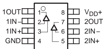
TLV2462 D OR PW PACKAGE (TOP VIEW)
