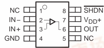
TLV2460 D OR PW PACKAGE (TOP VIEW)
