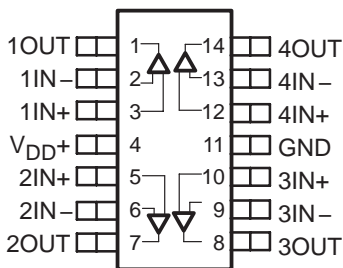
TLV2464 D OR PW PACKAGE (TOP VIEW)
