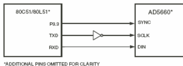
Figure 29. AD5660 to 80C51 Interface
