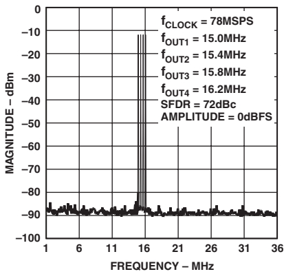
TPC 15. Four-Tone SFDR
