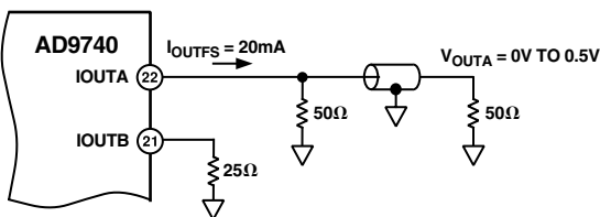
Figure 13. 0 V to 0.5 V Unbuffered Voltage Output
