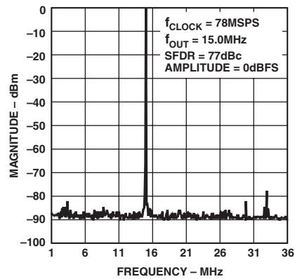
TPC 13. Single-Tone SFDR
