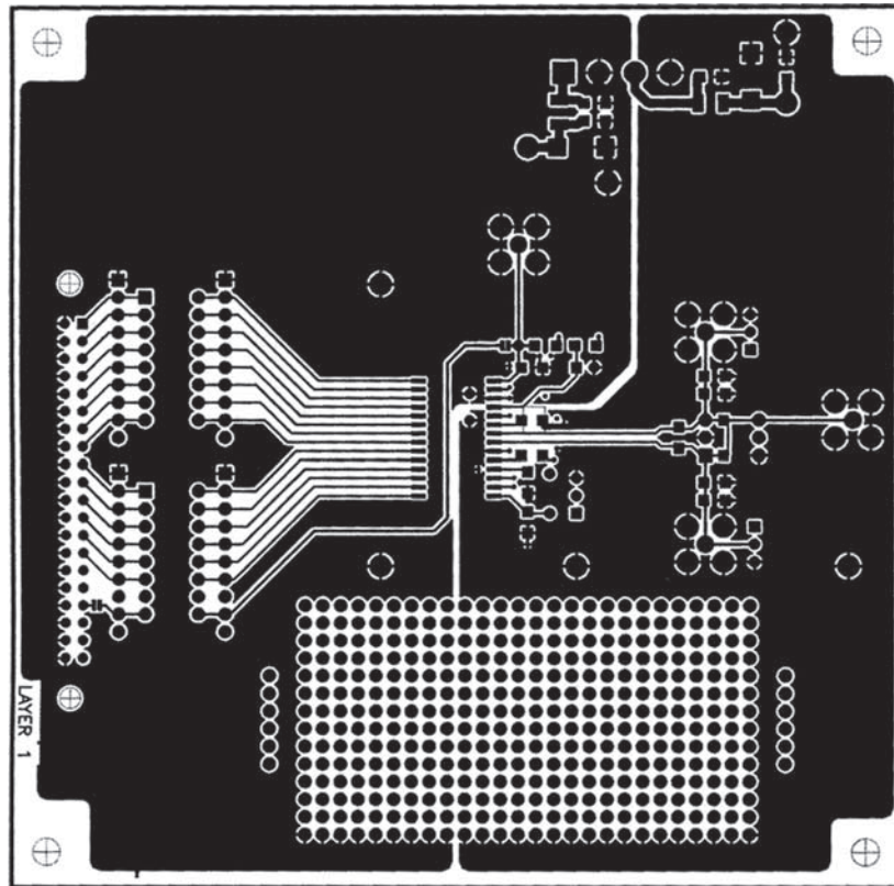
Figure 19. Primary Side
