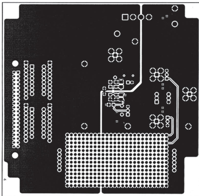
Figure 20. Secondary Side
