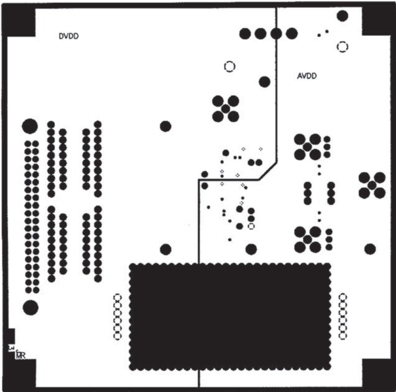
Figure 22. Power Plane
