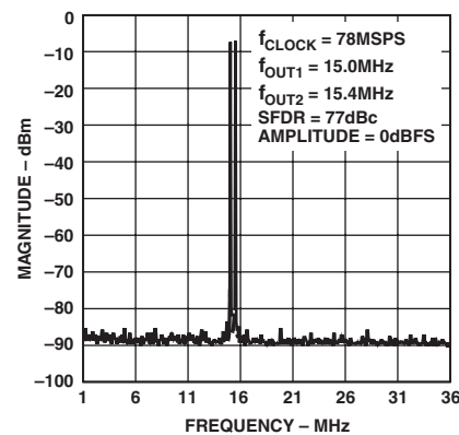
TPC 14. Dual-Tone SFDR
