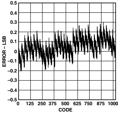
Figure 15. Typical INL
