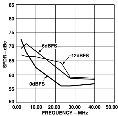
Figure 25. SFDR vs. f_{OUT} @ 100 MSPS
