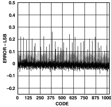
Figure 16. Typical DNL
