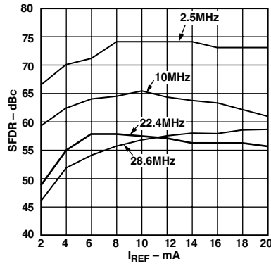
Figure 31. SFDR vs. f_{\text{OUT}} and I_{\text{OUTFS}} @ 100 MSPS, 0 dBFS
