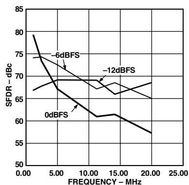
Figure 24. SFDR vs. f_{OUT} @ 50 MSPS
