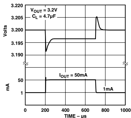
Figure 14. Load Transient
