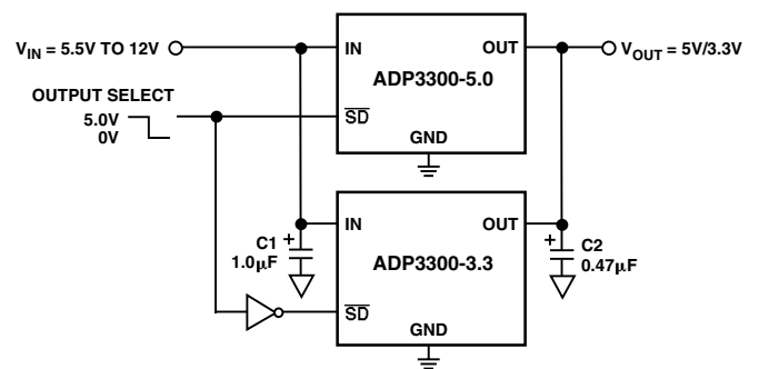
Figure 22. Crossover Switch
