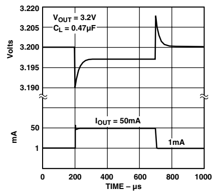
Figure 13. Load Transient
