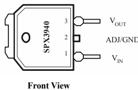
TO-252 Package
