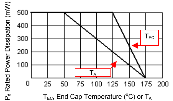
T_{EC} , End Cap Temperature (°C) or T_A Ambient temperature on FR4 PC board FIGURE 2 Power Derating Curve
