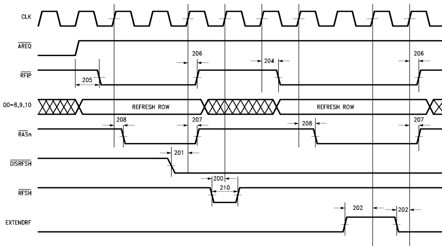
FIGURE 39. 200: Refresh Timing
