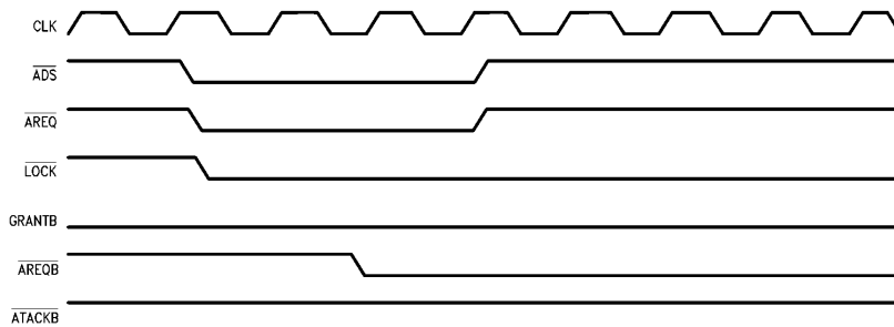
FIGURE 35. \overline{\text{LOCK}} Function
