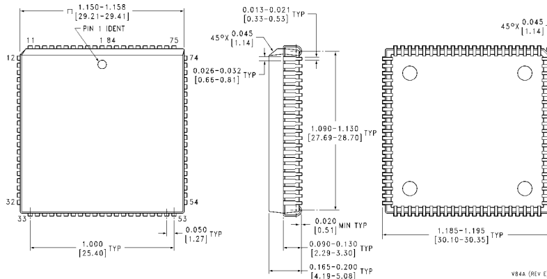
Plastic Chip Carrier (V) Order Number DP8422AV-20 or DP8422AV-25 NS Package Number V84A
