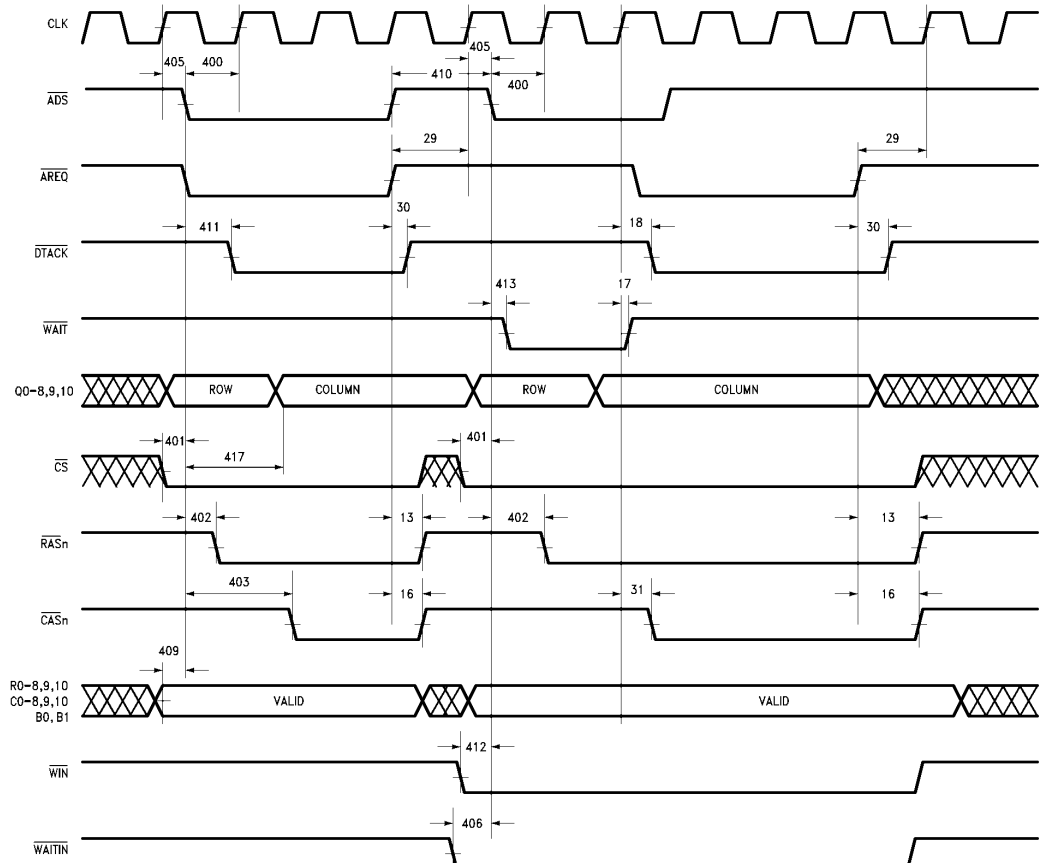
FIGURE 42. 400: Mode 1 Timing
