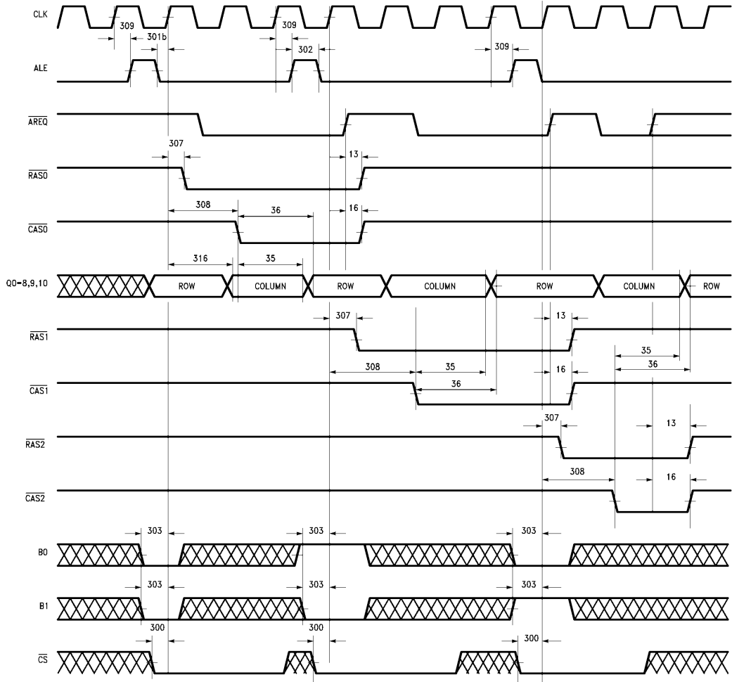
FIGURE 41. 300: Mode 0 Interleaving
