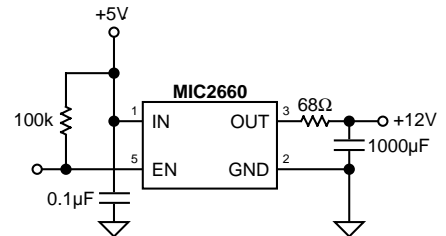
Figure 2. Charge-Pump/Dump
