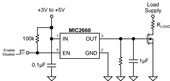
Figure 1. Charge-Pump Driver
