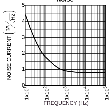
Current Noise
