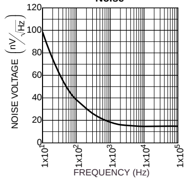
Voltage Noise
