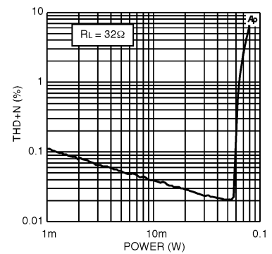
Headphone Amplifier THD+N vs Output Power
