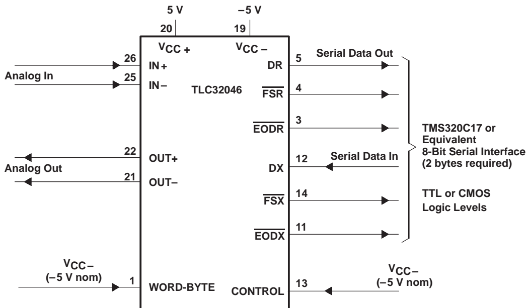
Figure 1–3. Byte Mode
