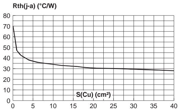
Fig. 11: Thermal resistance junction to ambient versus copper surface under tab (Epoxy printed circuit board FR4, copper thickness: 35µm) (D 2 PAK).
