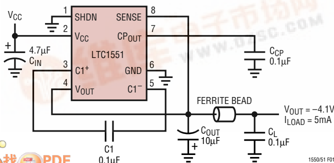
-4.1V Generator with 1mV P-P Noise
