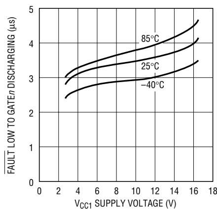
FAULT Low to GATE \bar{n} Discharging vs V_{CC1} Supply Voltage
