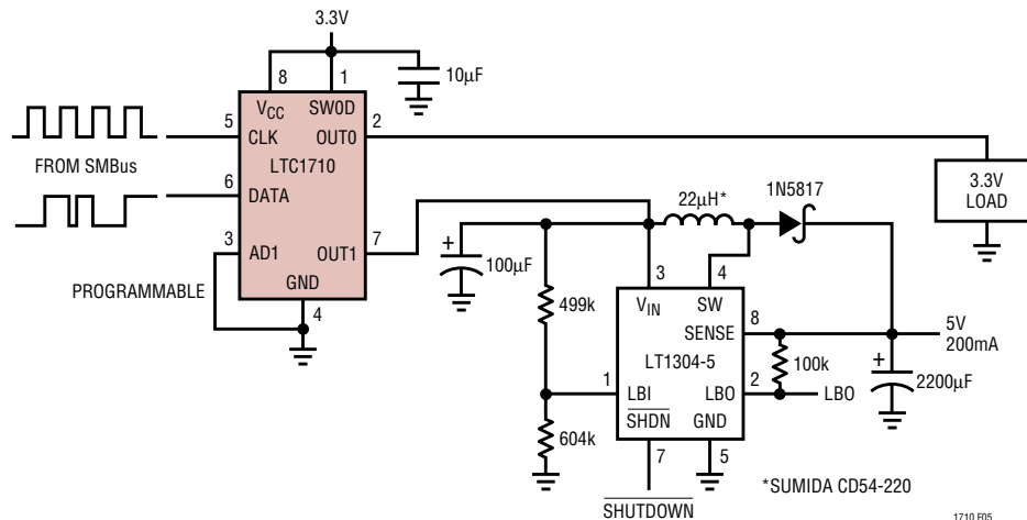
Figure 5. Switching Regulator with Low-Battery Detect Using 22 \mu A of Standby Current
