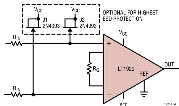
Figure 4. Input Protection
