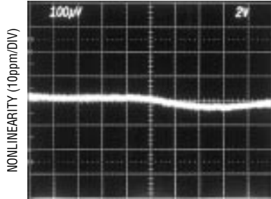
Gain Nonlinearity, G = 10
