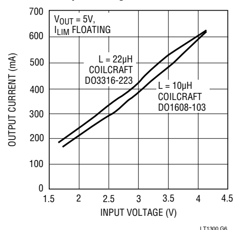
Maximum Output Current vs Input Voltage
