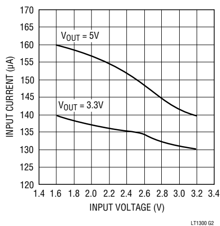
No-Load Battery Current
