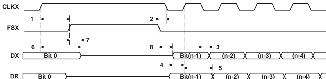
Figure 4–46. McBSP Timing as SPI Master or Slave: CLKSTP = 10b, CLKXP = 1
