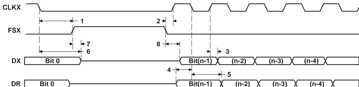
Figure 4–44. McBSP Timing as SPI Master or Slave: CLKSTP = 10b, CLKXP = 0
