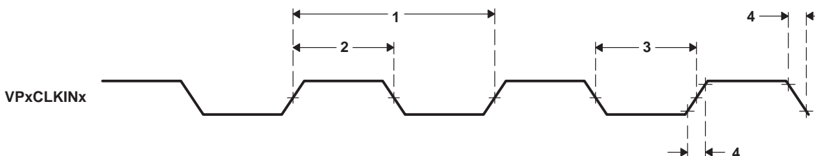
Figure 4–48. Video Port Capture VPxCLKINx Timing
