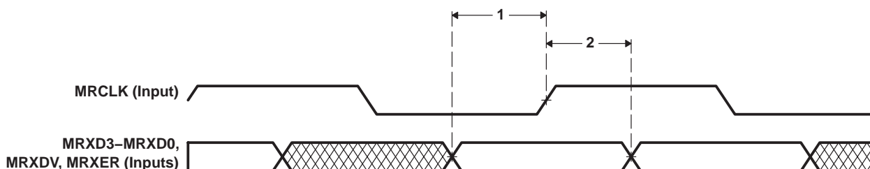
Figure 4–56. EMAC Receive Interface Timing
