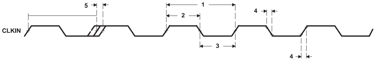
Figure 4–11. CLKIN Timing
