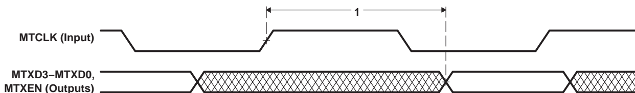
Figure 4–57. EMAC Transmit Interface Timing
