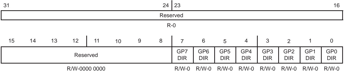
Figure 4–62. GPIO Direction Register (GPDIR) [Hex Address: 01B0 0004]
