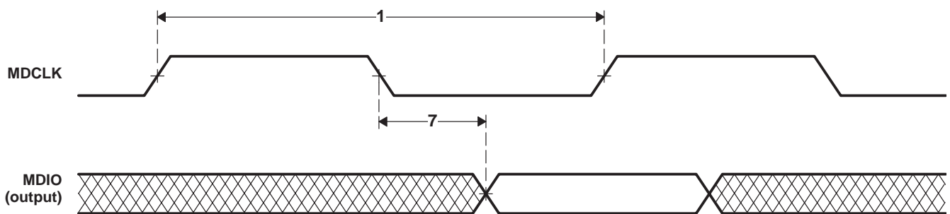
Figure 4-59. MDIO Output Timing
