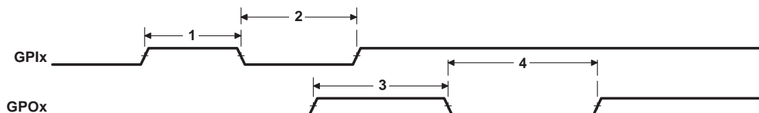
Figure 4–63. GPIO Port Timing
