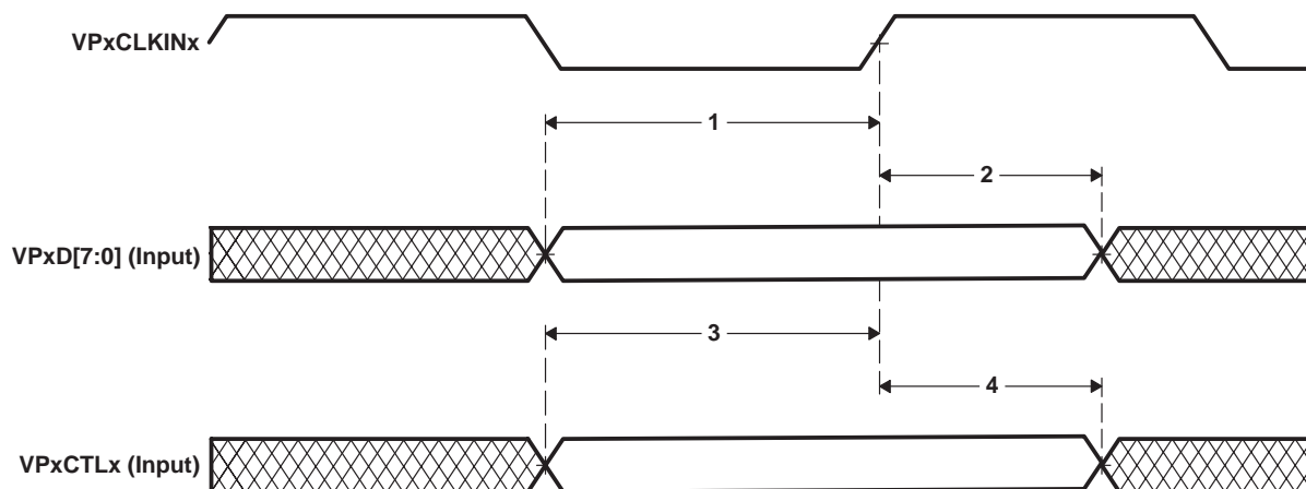
Figure 4–49. Video Port Capture Data and Control Input Timing
