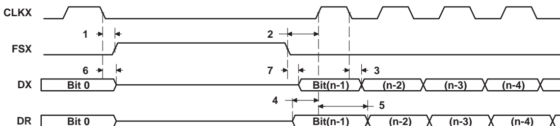
Figure 4–45. McBSP Timing as SPI Master or Slave: CLKSTP = 11b, CLKXP = 0
