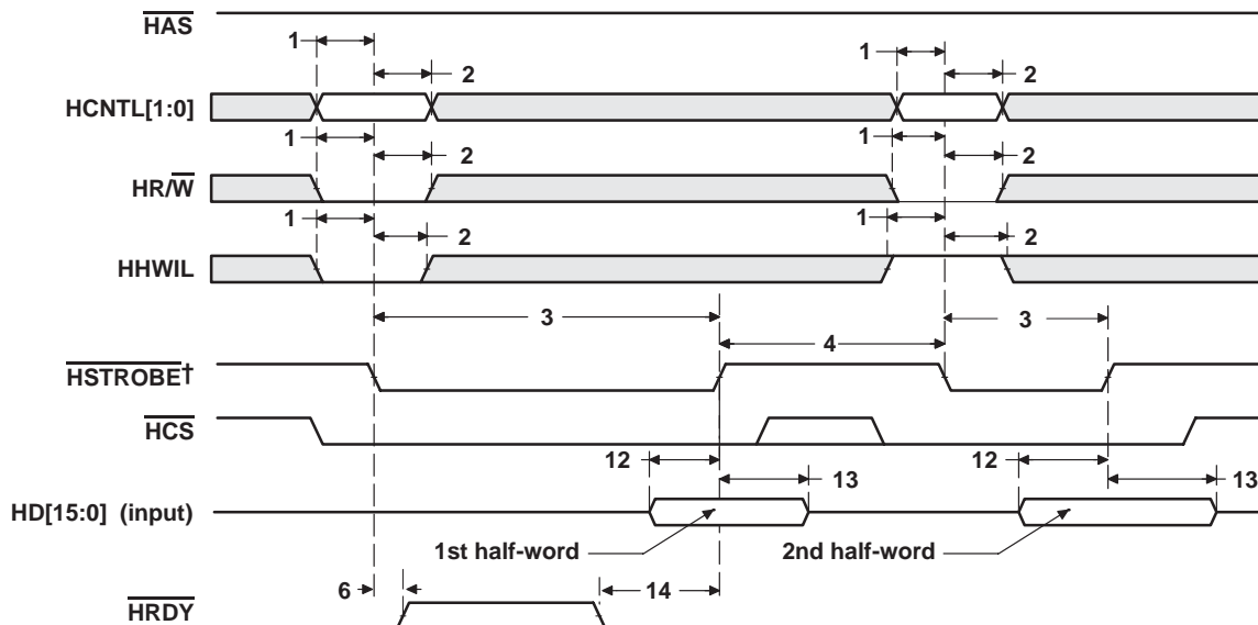
Figure 4–40. HPI16 Write Timing ( \overline{\text{HAS}} Not Used, Tied High) [DM641 Only]
