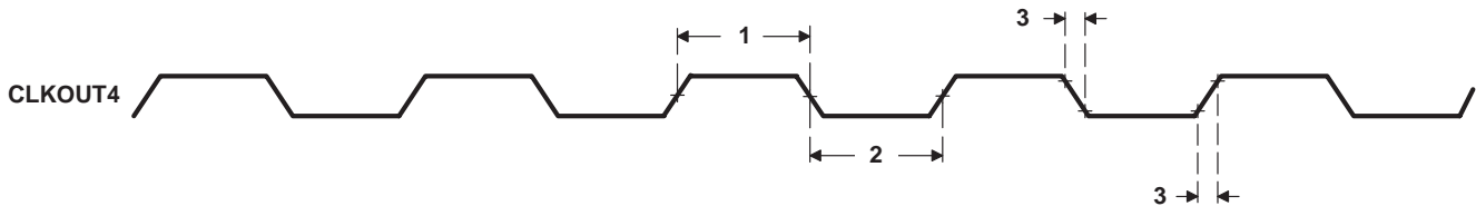
Figure 4–12. CLKOUT4 Timing
