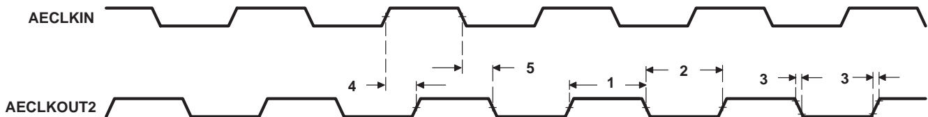
Figure 4–16. AECLKOUT2 Timing for the EMIFA Module
