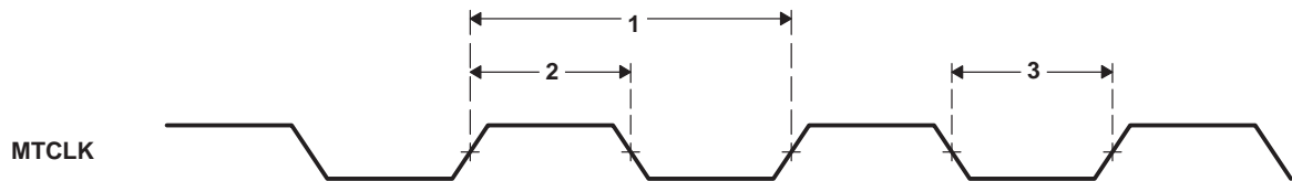
Figure 4–55. MTCLK Timing (EMAC – Transmit)
