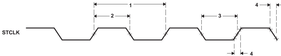
Figure 4–53. STCLK Timing
