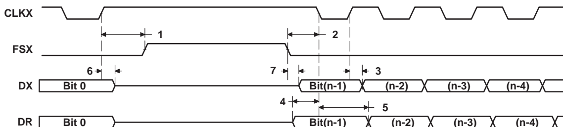
Figure 4–47. McBSP Timing as SPI Master or Slave: CLKSTP = 11b, CLKXP = 1
