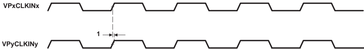
Figure 4–52. Video Port Dual-Display Sync Timing
