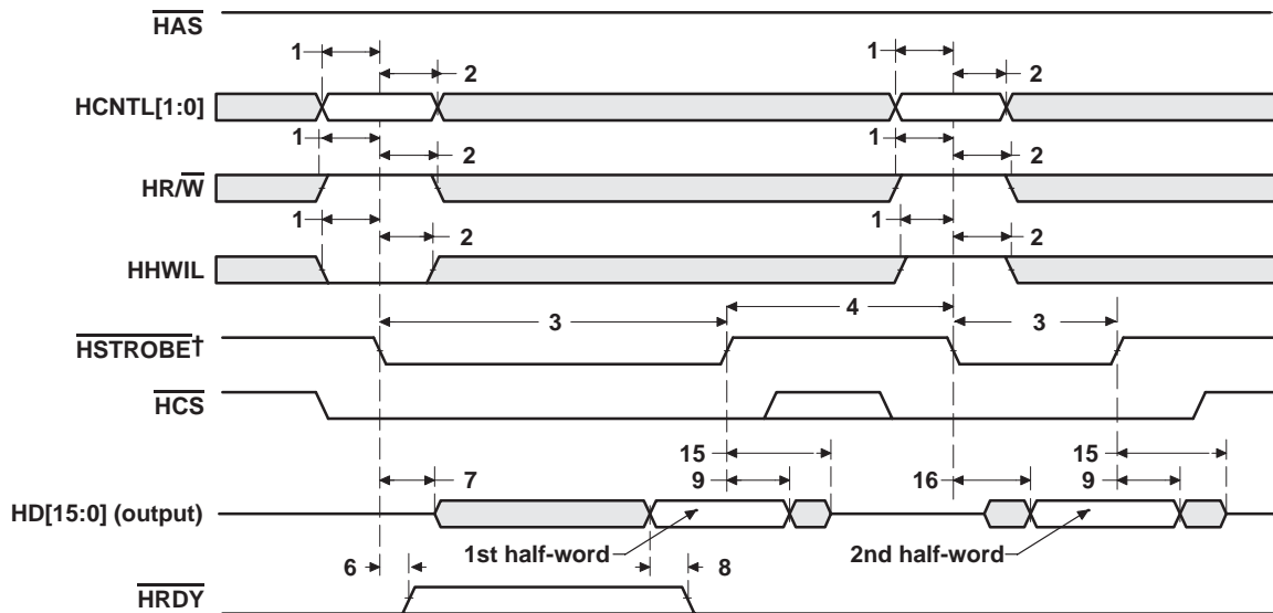
Figure 4–38. HPI16 Read Timing (HAS Not Used, Tied High) [DM641 Only]
