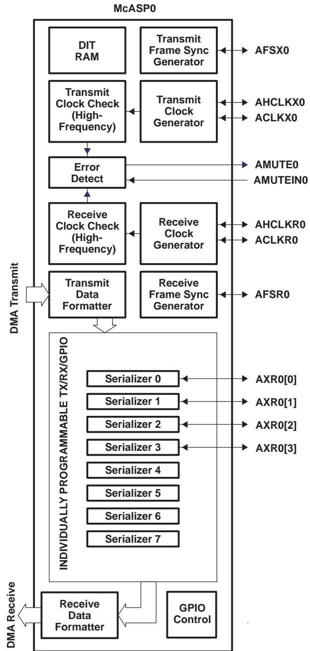
Figure 4-32. McASP0 Configuration
