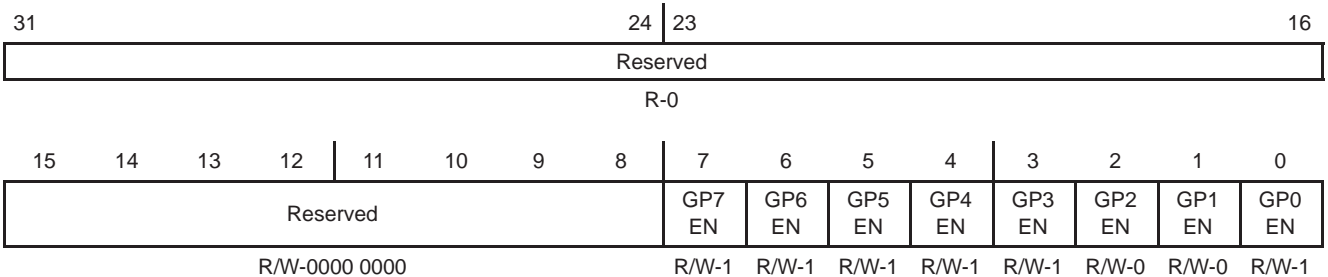
Figure 4–61. GPIO Enable Register (GPEN) [Hex Address: 01B0 0000]
