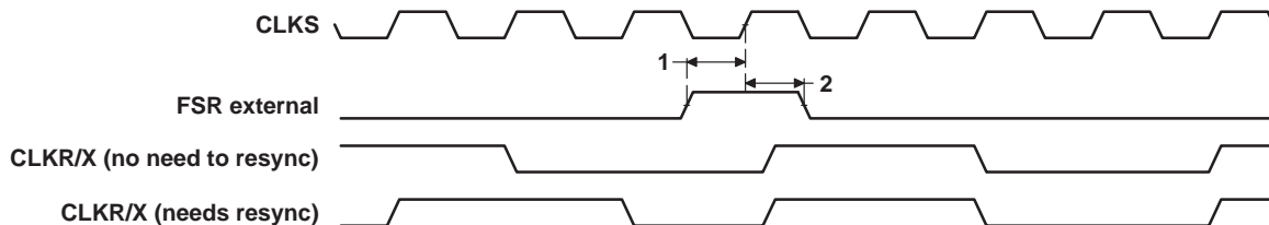
Figure 4–43. FSR Timing When GSYNC = 1
