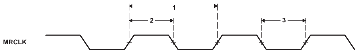
Figure 4–54. MRCLK Timing (EMAC – Receive)
