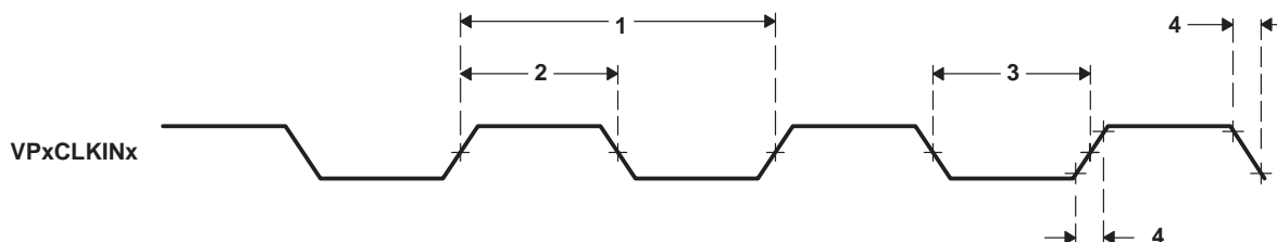
Figure 4–50. Video Port Display VPxCLKINx Timing
