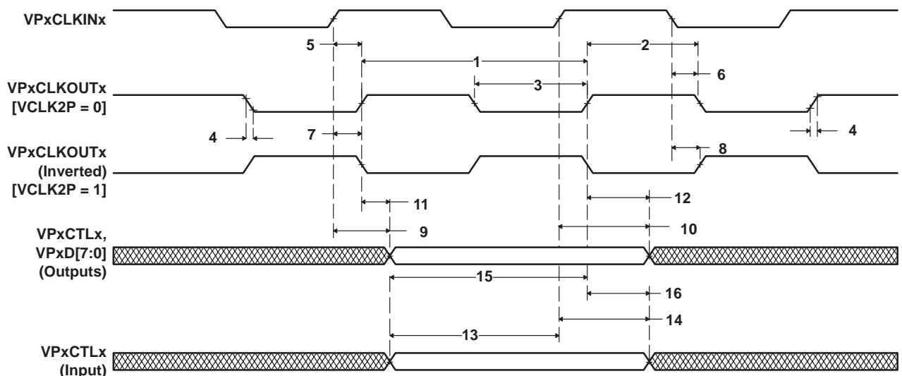
Figure 4–51. Video Port Display Data Output Timing and Control Input/Output Timing With Respect to VPxCLKINx and VPxCLKOUTx
