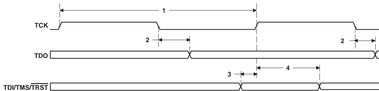
Figure 4–65. JTAG Test-Port Timing
