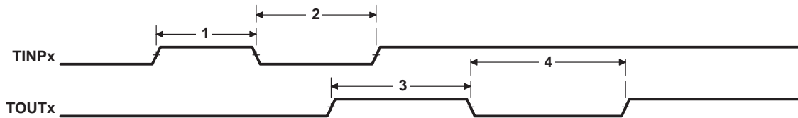
Figure 4-60. Timer Timing
