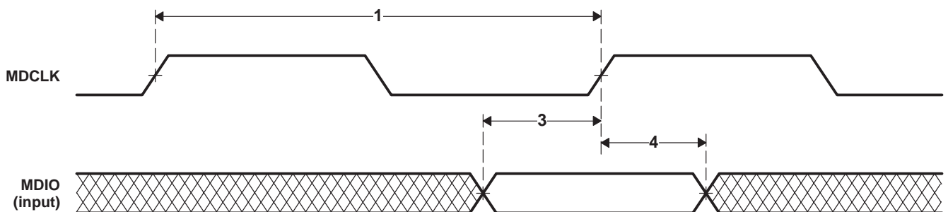
Figure 4-58. MDIO Input Timing
