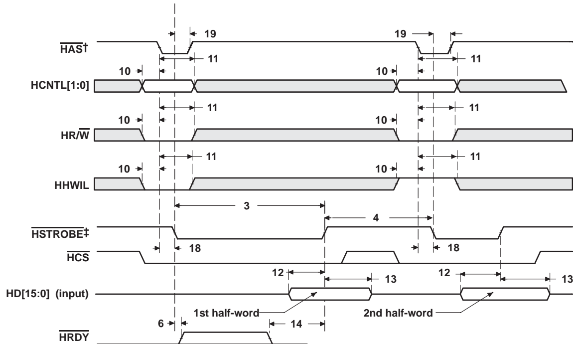
Figure 4–41. HPI16 Write Timing ( \overline{\text{HAS}} Used) [DM641 Only]
