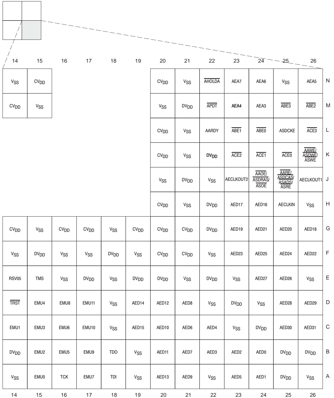
Figure 1–4. DM641/DM640 Pin Map (Continued) [Quadrant D]
