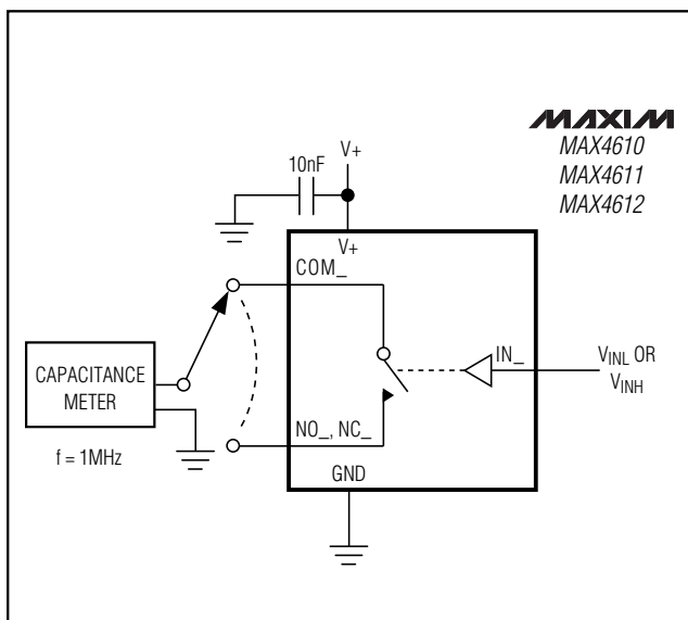
Figure 6. Channel Off/On-Capacitance
