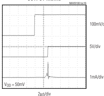
SWITCHING CURRENT, OUTPUT RISING
