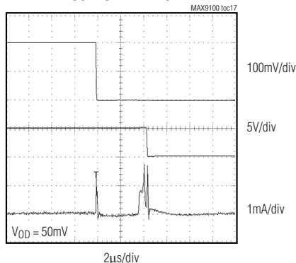
SWITCHING CURRENT, OUTPUT FALLING
