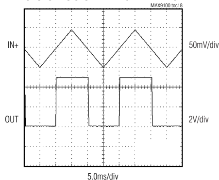
RESPONSE TO SLOW TRIANGLE WAVEFORM
