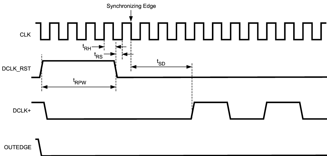
FIGURE 7. Clock Reset Timing in SDR Mode with \text{OUTEDGE} Low
