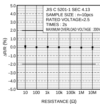
Fig.9 Overload
