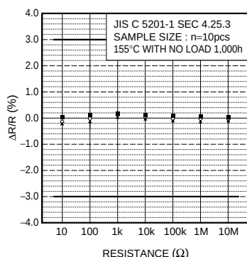
Fig.15 Endurance
