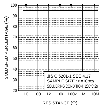
Fig.10 Solderability
