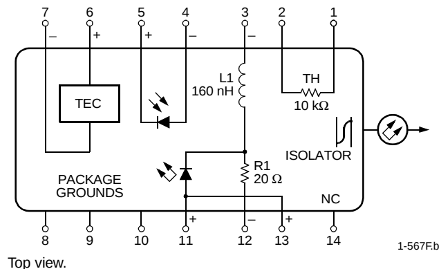
Figure 1. Circuit Schematic
